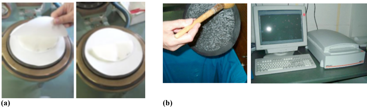
Figure 1: Determination of flake content (a) and macrosticky content (b) [12]
